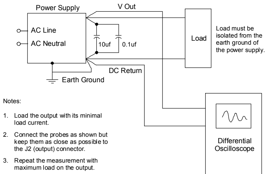
Figure 3-7 Ripple Noise Measurement Setup
