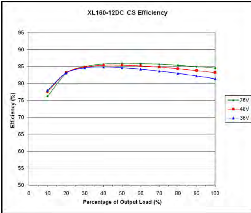
Figure 5-19 Efficiency of XL160-12DC CS (Current Sharing)
