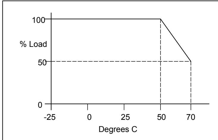
Figure 3-1 Derating Curve for Elevated Temperature Operation
