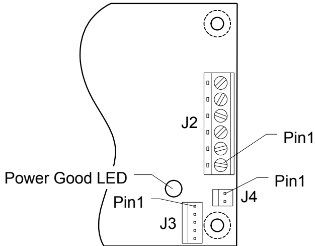
Figure 4-5 XL160-05DC [CS] Output Connectors Layout
