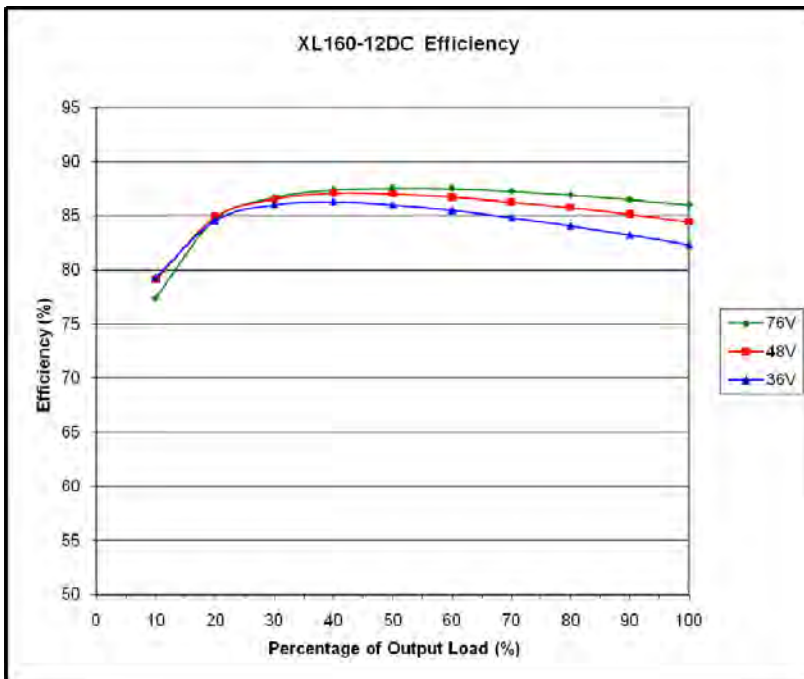
Figure 5-20 Efficiency of XL160-12DC (Non Current Sharing)
