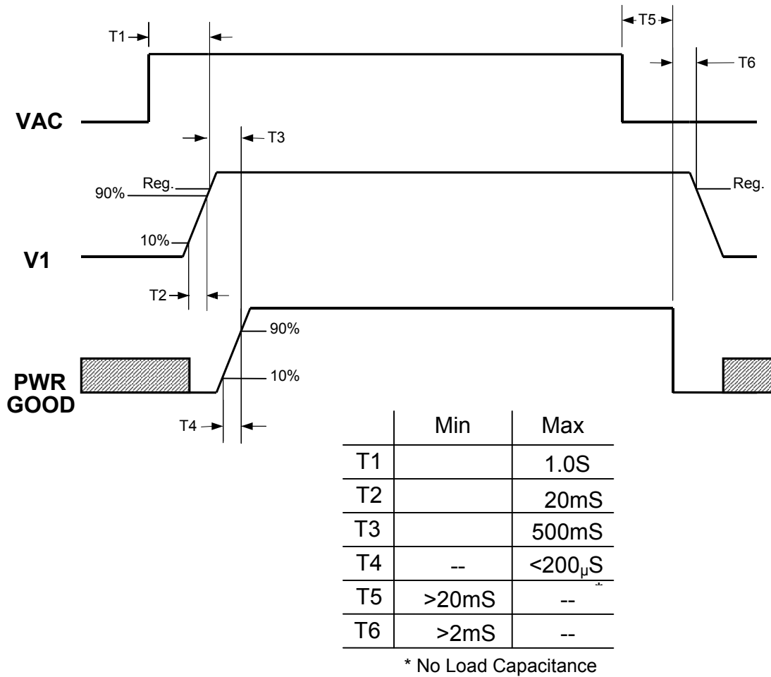
Figure 6-1 Timing Diagram
