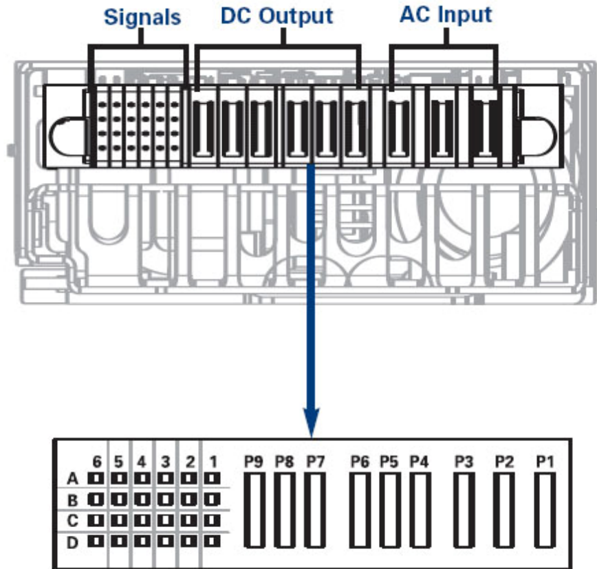
Rear View of Rectifier
