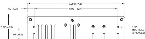
ALL DIMENSIONS IN INCHES (MM)
