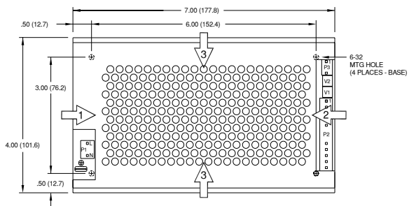
OPTIONAL COVER
